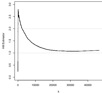
Figure 15: Hill estimator for interarrival times
