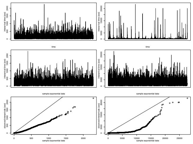
Figure 12: Fitting an exponential distribution to interarrival times
